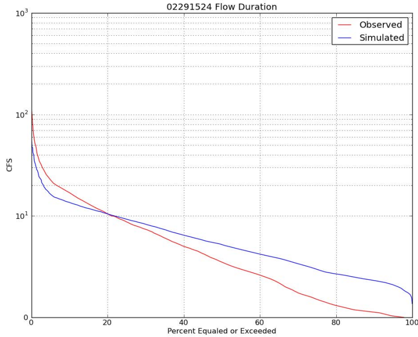
Figure 5-10. USGS 02291524 (Spring Creek) Flow Duration Plot
