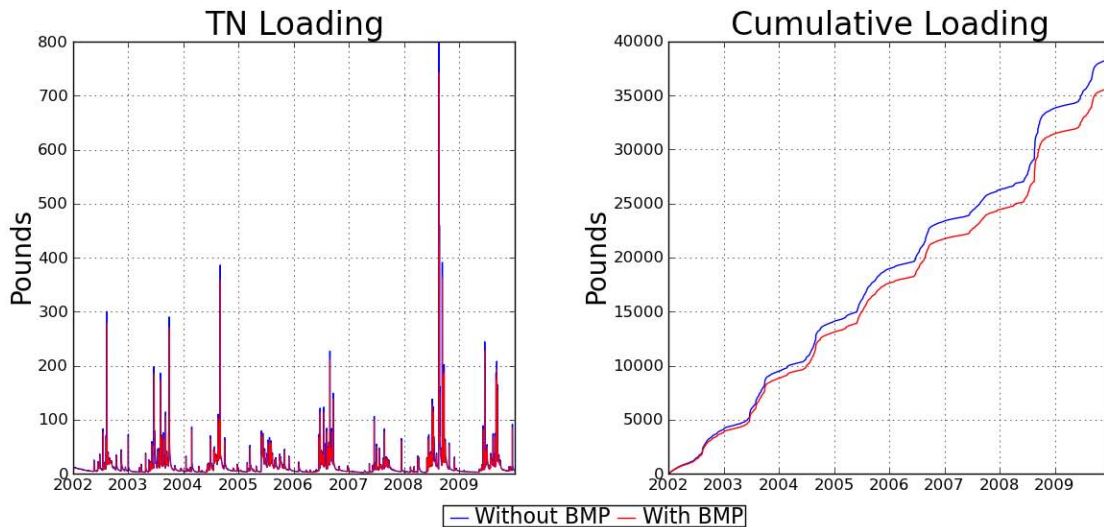
Figure 7-23. HSPF Simulated TN Removal, BMP 3
